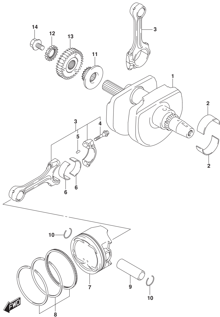
DL650M5_E01_120A CRANKSHAFT
