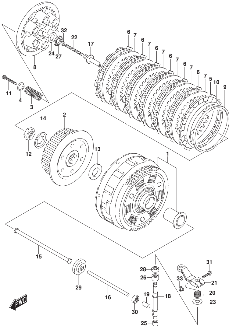
DL650M5_E01_201A CLUTCH
