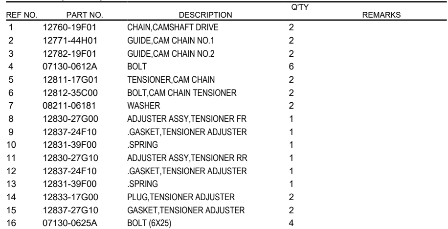
FIG.127A (1-B-12) CAM CHAIN
