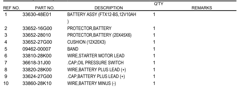
FIG.310D (1-C-15) BATTERY
