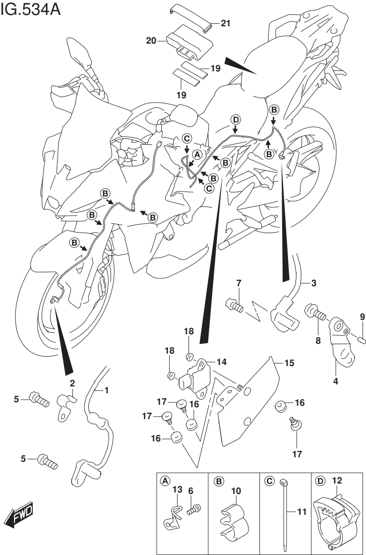
FIG.534A (1-G-10) BODY ELECTRICAL
