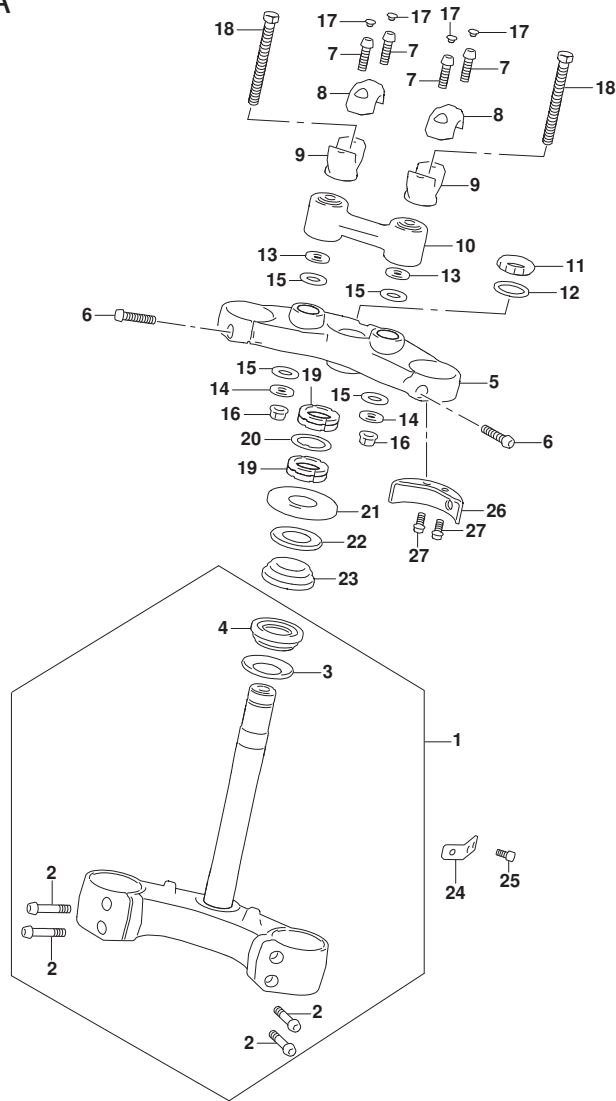
FIG.524A (1-G-7) STEERING STEM
