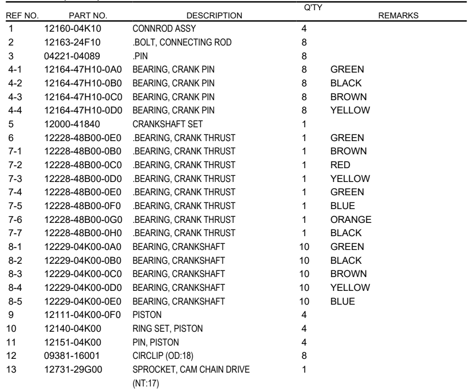
FIG.120A (1-B-9) CRANKSHAFT
