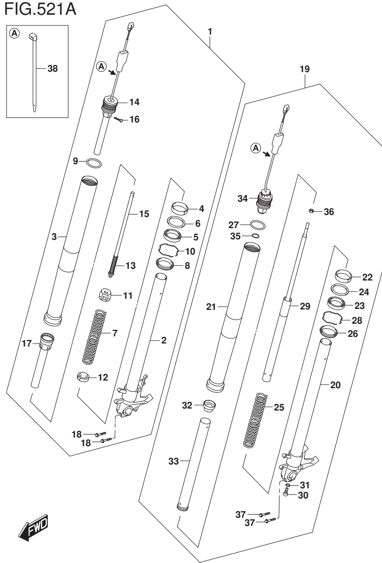
FIG.521A (1-G-5) FRONT FORK DAMPER
