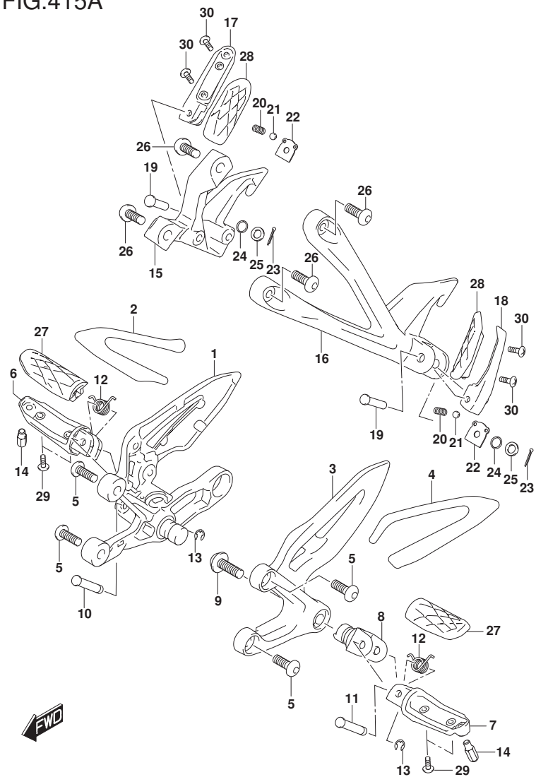
GSX-S1000TRQM4_E21_415A FOOTREST
