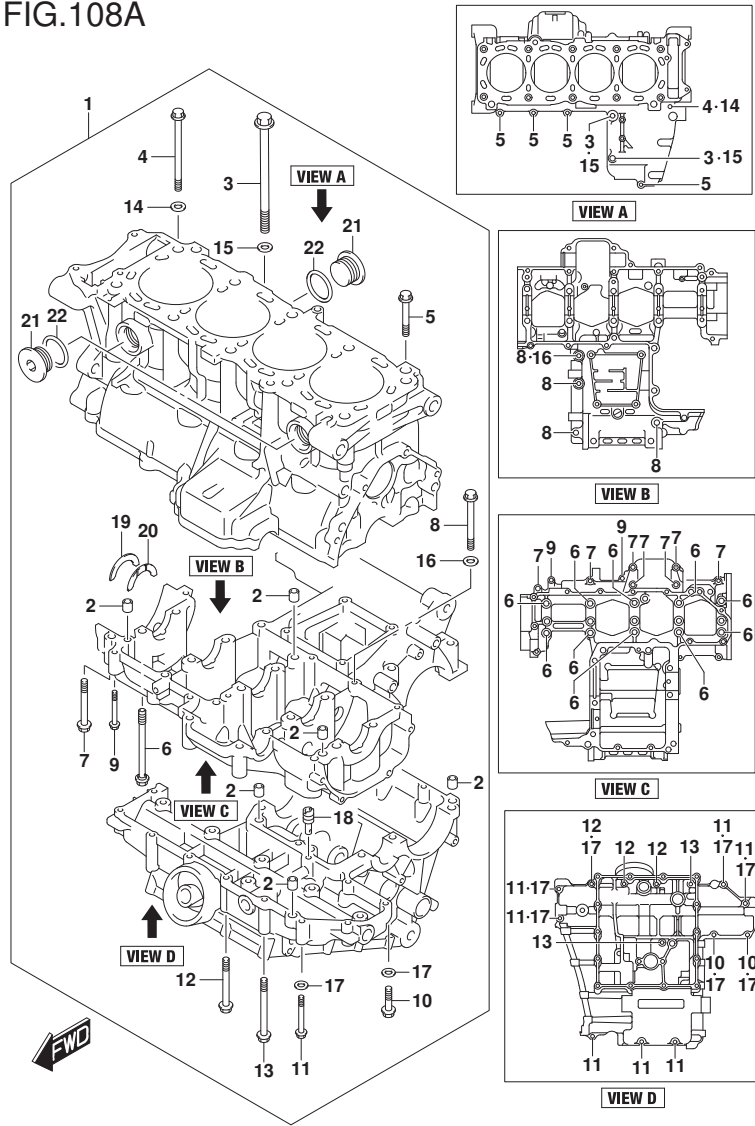
FIG.108A (1-B-5) CRANKCASE
