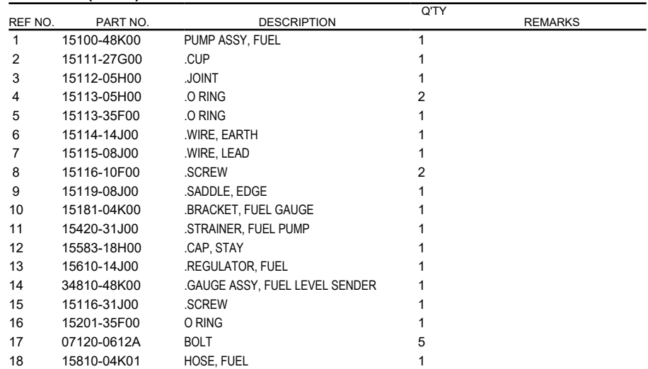
FIG.172A (1-C-4) FUEL PUMP
