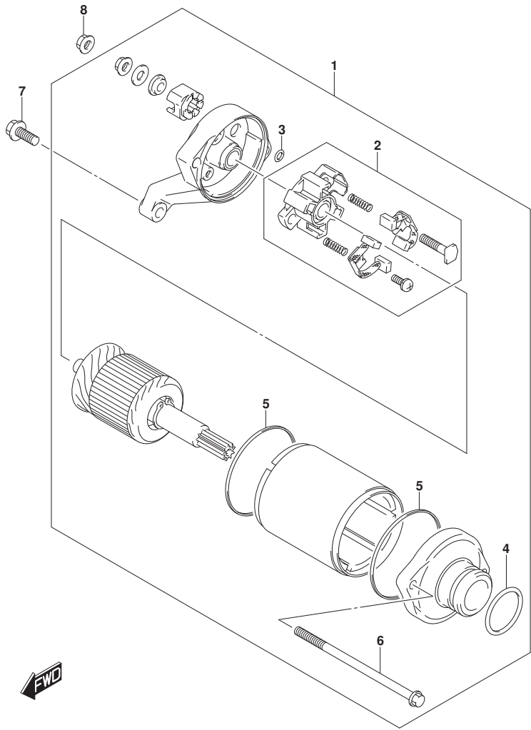
SV650M5_E11_301A STARTING MOTOR
