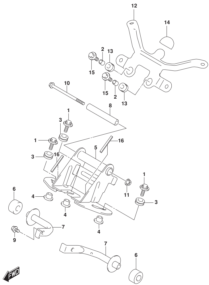
DL1050M5_E21_444A FRONT BRACKET
