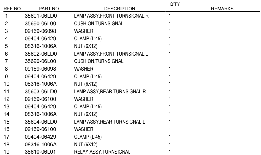
FIG.334A (1-D-15) TURNSIGNAL LAMP (DL1050RJ)
