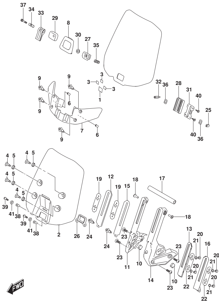
DL1050M5_E21_454C WINDSCREEN
