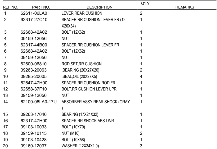
FIG.543A (1-I-10) REAR CUSHION LEVER (DL1050RJ)
