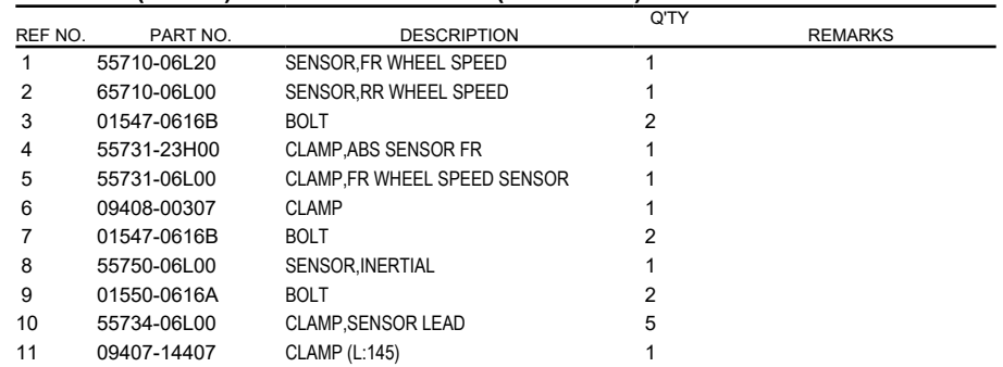
FIG.534A (1-H-15) BODY ELECTRICAL (DL1050RR)
