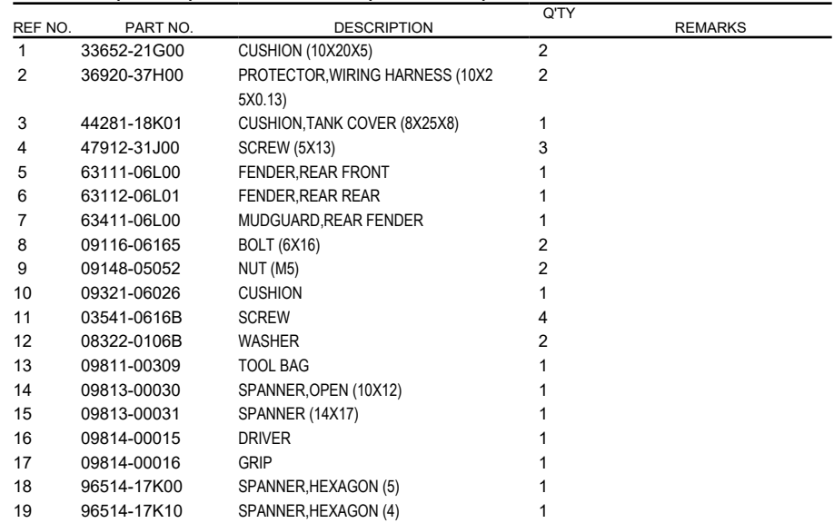
FIG.474A (1-G-10) REAR FENDER (DL1050RR)
