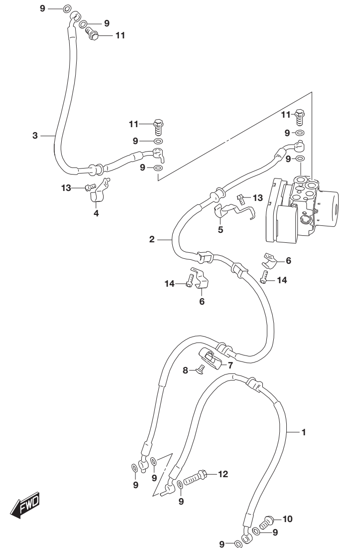
DL800DEM5_E21_536A FRONT BRAKE HOSE
