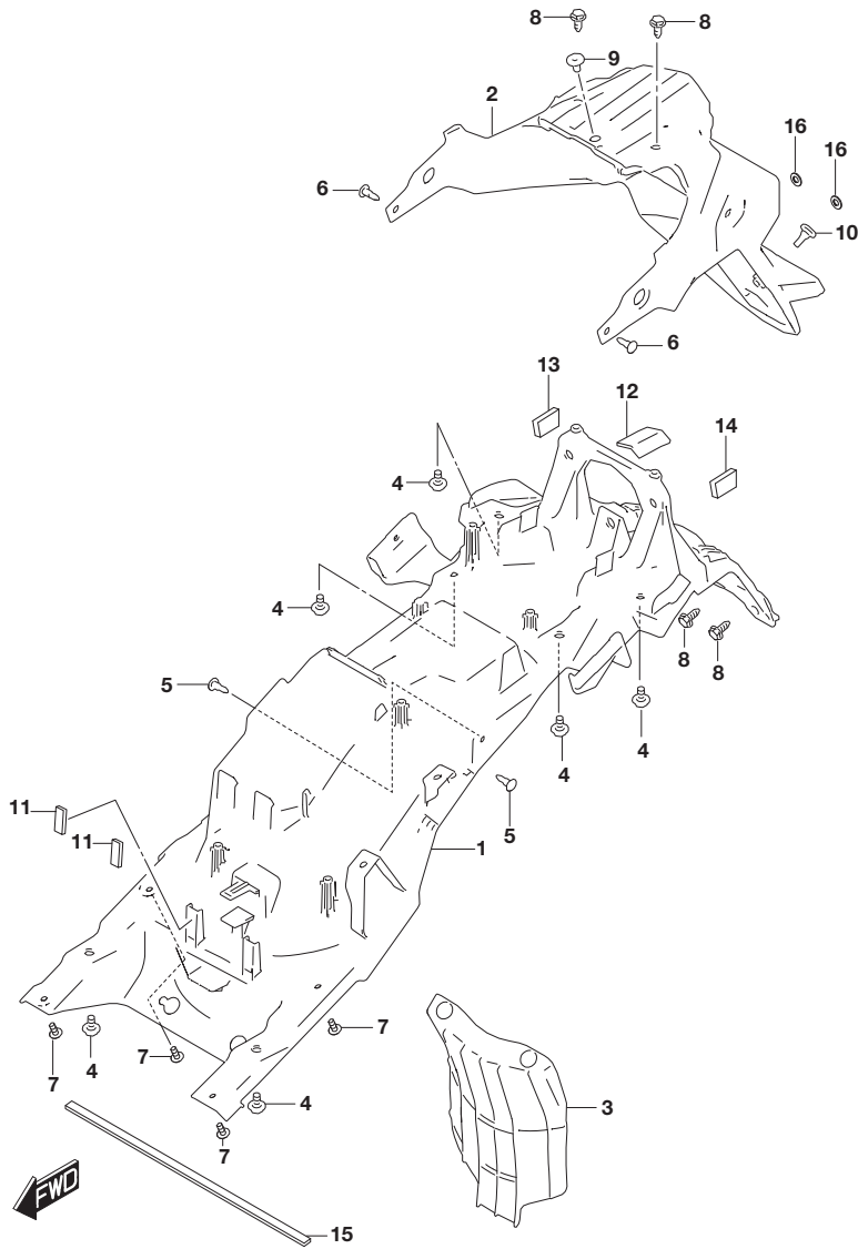
FIG.474A (1-F-11) REAR FENDER
