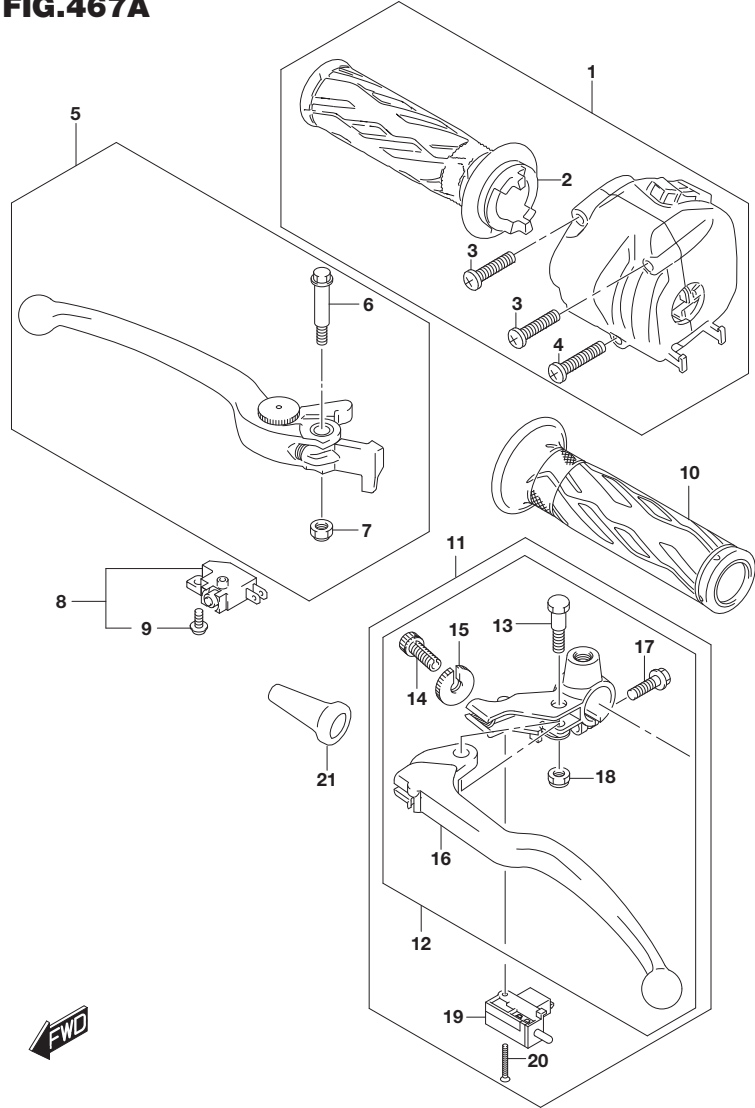
DL800DEM5_E21_467A HANDLE LEVER
