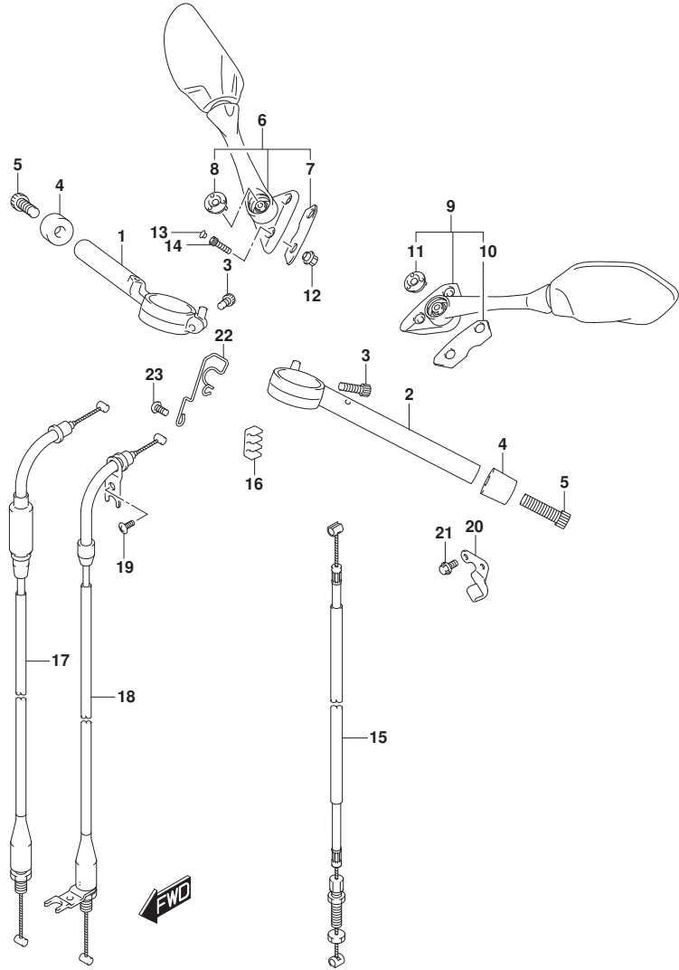
GSX-R1000M5_E06_462A HANDLEBAR
