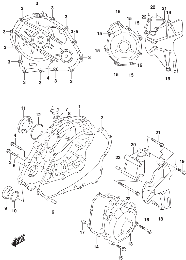
GSX-R1000M5_E06_112A CRANKCASE COVER
