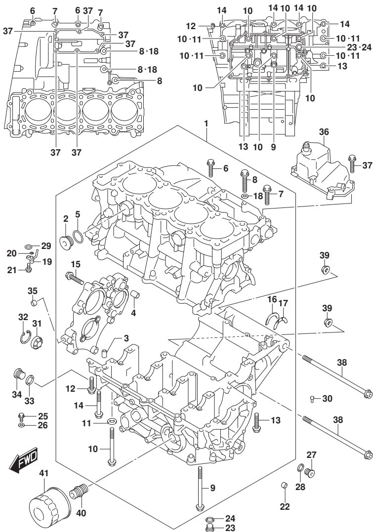
GSX-R1000M5_E06_108A CRANKCASE
