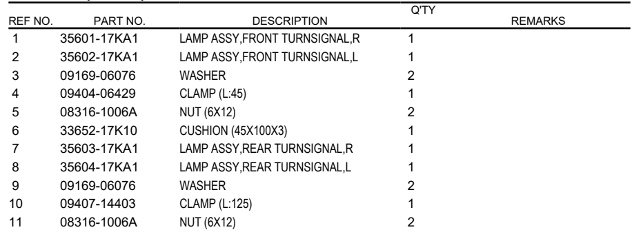
FIG.334B (1-D-11) TURNSIGNAL LAMP
