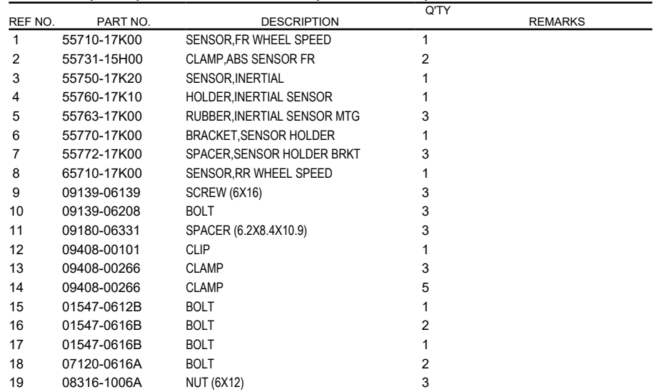
FIG.534A (1-H-3) BODY ELECTRICAL (GSX-R1000A)
