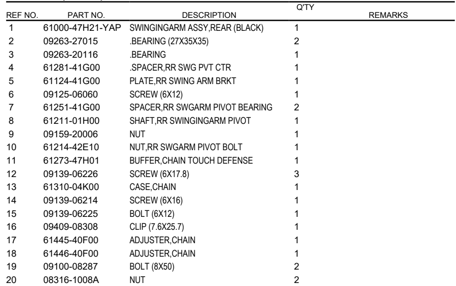
FIG.541A (1-F-12) REAR SWINGINGARM
