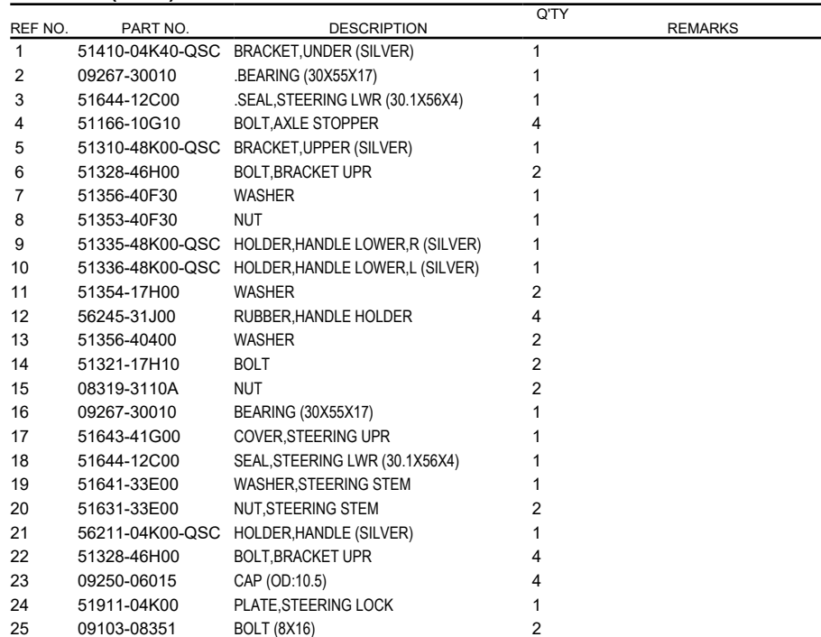
FIG.524A (1-F-5) STEERING STEM
