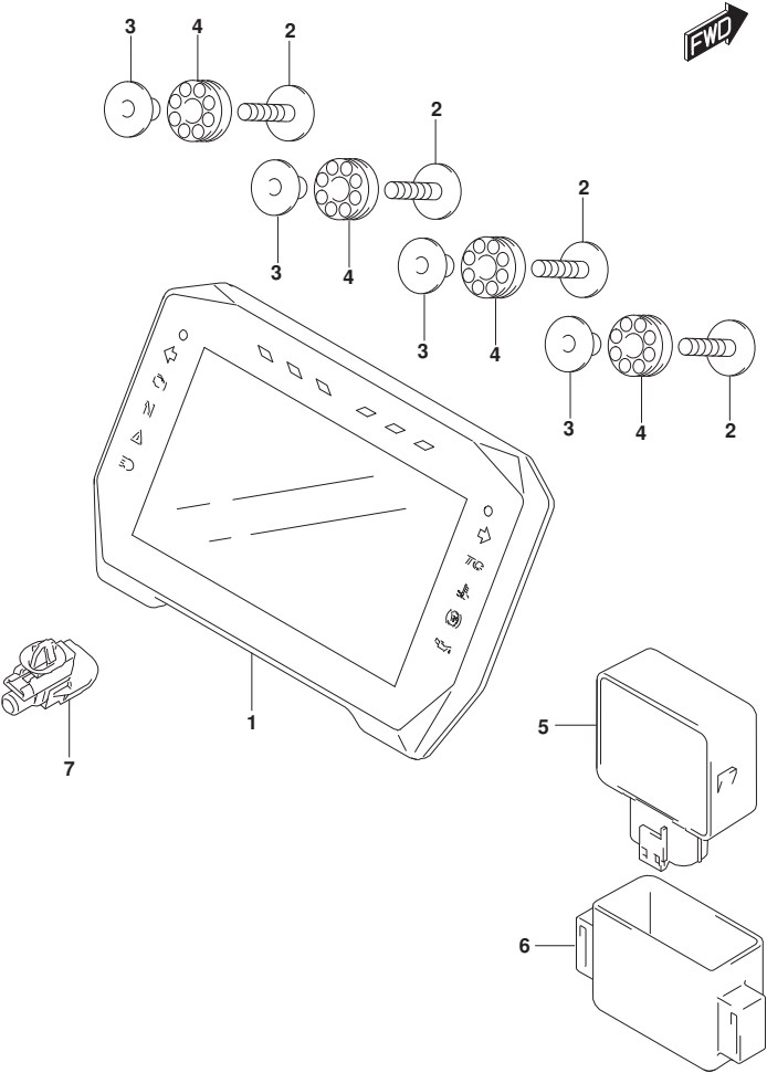
GSX-S1000TM5_E21_330A SPEEDOMETER
