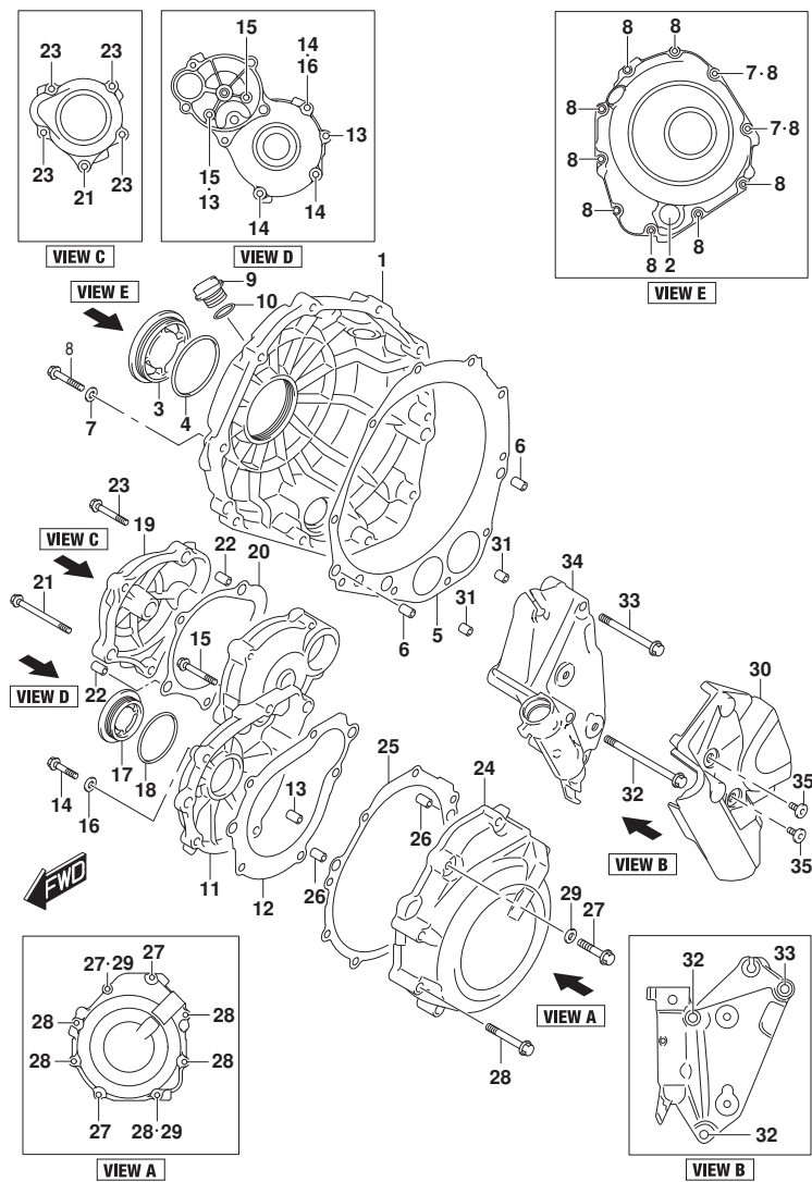
GSX-S1000TM5_E21_112A CRANKCASE COVER
