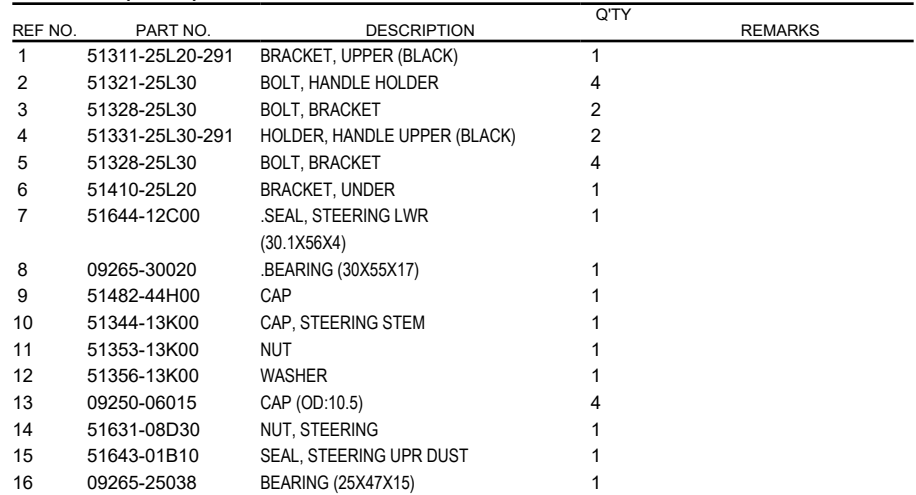
FIG.524A (1-G-4) STEERING STEM
