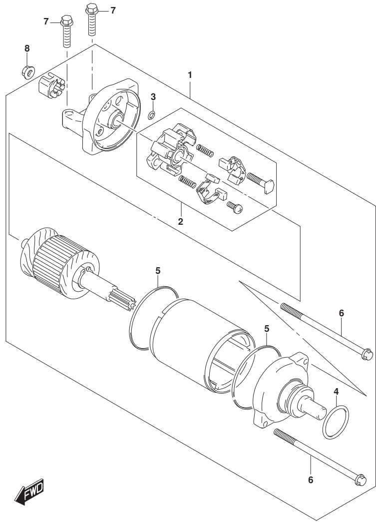
DL800M5_E21_301A STARTING MOTOR
