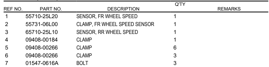
FIG.526A (1-G-5) SPEED SENSOR
