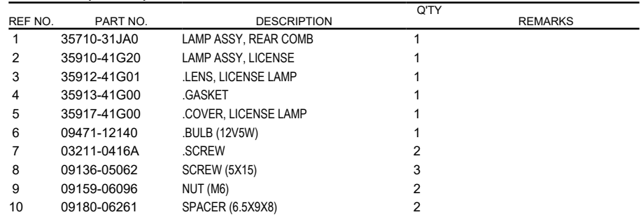
FIG.339A (1-D-14) REAR COMBINATION LAMP
