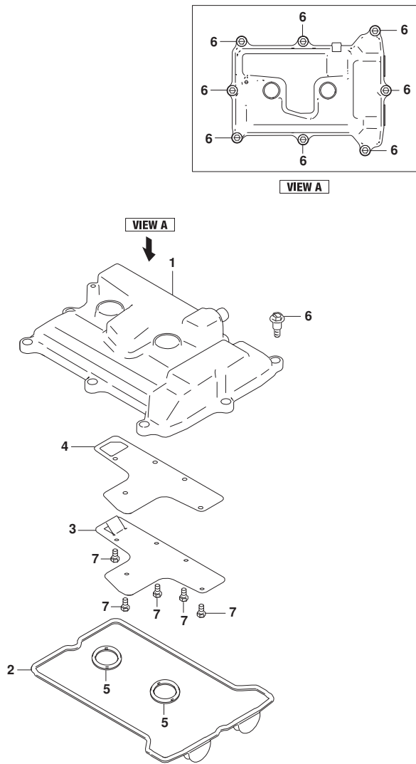
FIG.102A (1-B-3) CYLINDER HEAD COVER
