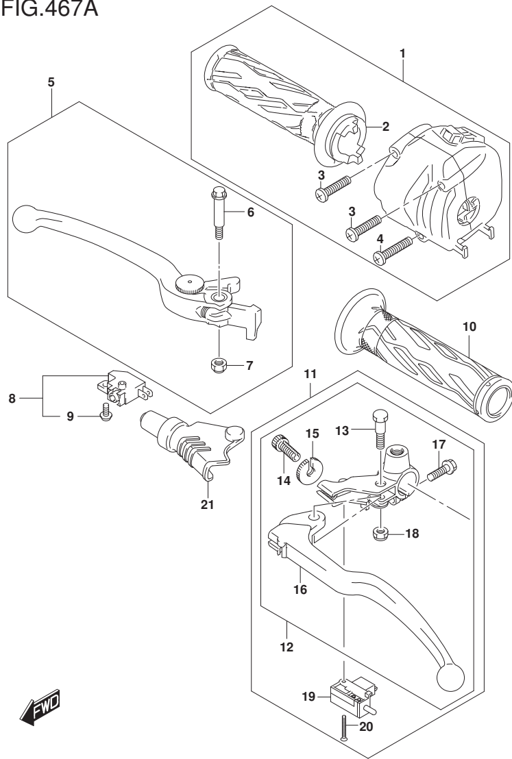
DL800M5_E21_467A HANDLE LEVER
