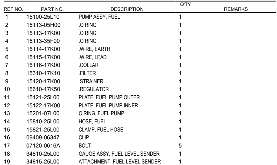
FIG.172A (1-C-6) FUEL PUMP
