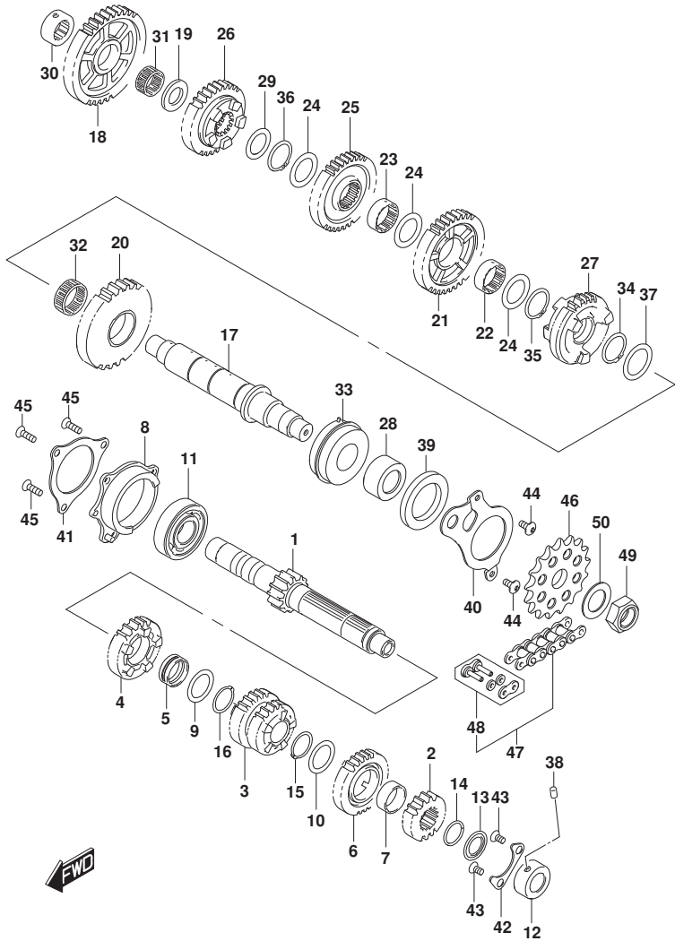
DL800M5_E21_206A TRANSMISSION
