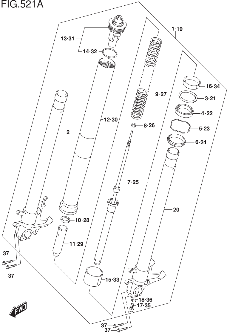
FIG.521A (1-F-7) FRONT FORK DAMPER
