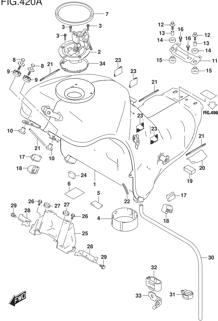
GSX-S1000SM5_E21_420A FUEL TANK
