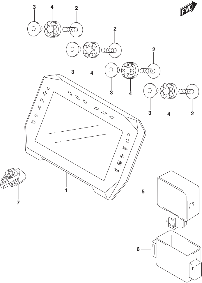
GSX-S1000TRQ2M3_E21_330A SPEEDOMETER
