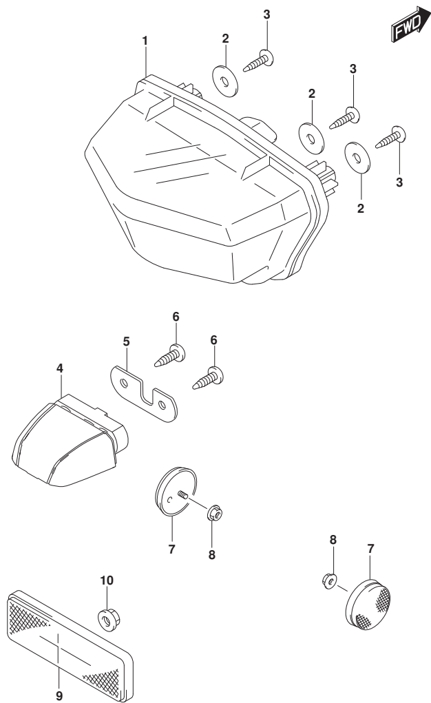
GSX-S1000TRQ2M3_E21_339A REARCOMBINATION LAMP
