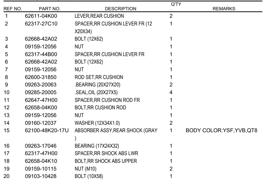
FIG.543A (1-F-12) REAR CUSHION LEVER
