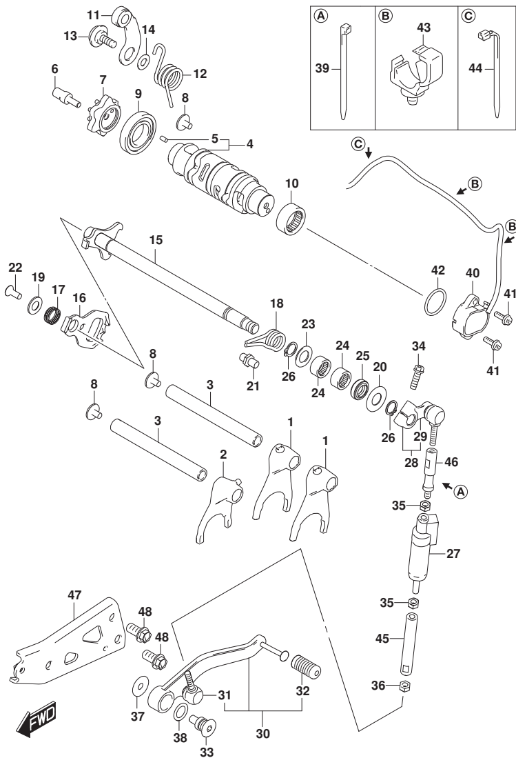
GSX800TM6_E21_212A GEAR SHIFTING
