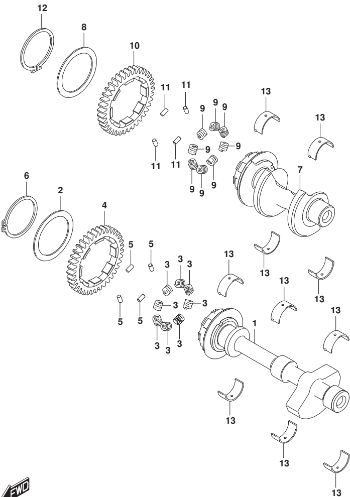
GSX800TM6_E21_124A CRANK BALANCER
