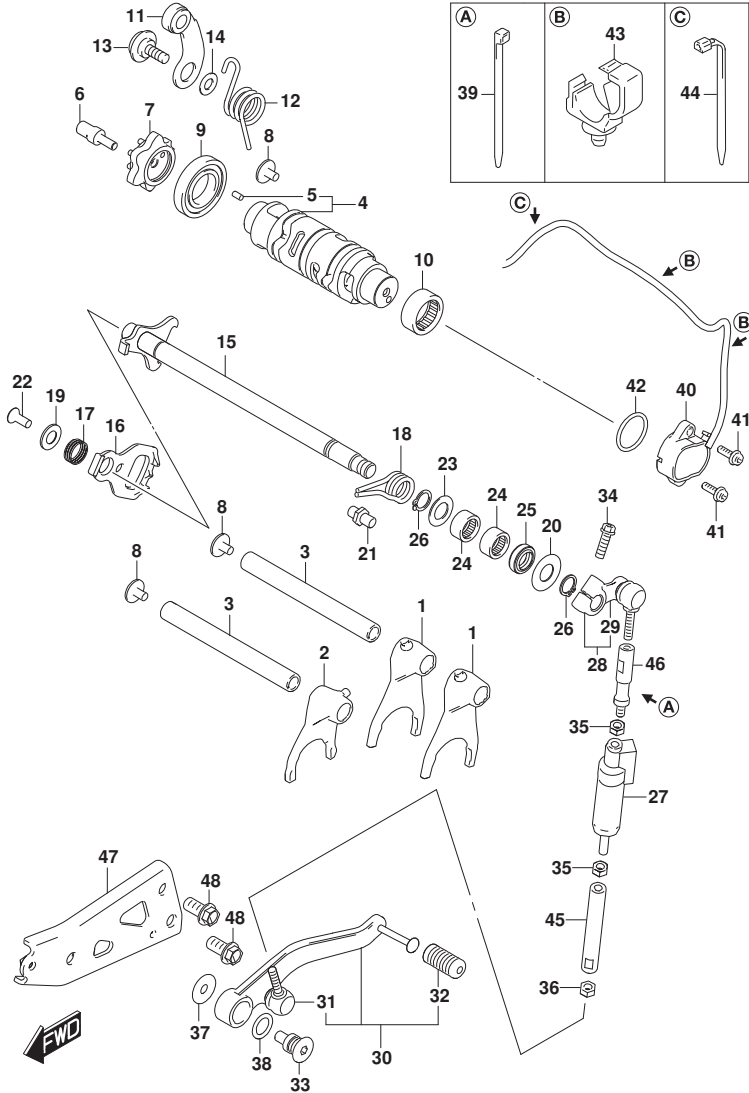
GSX800TM6_E21_212A GEAR SHIFTING
