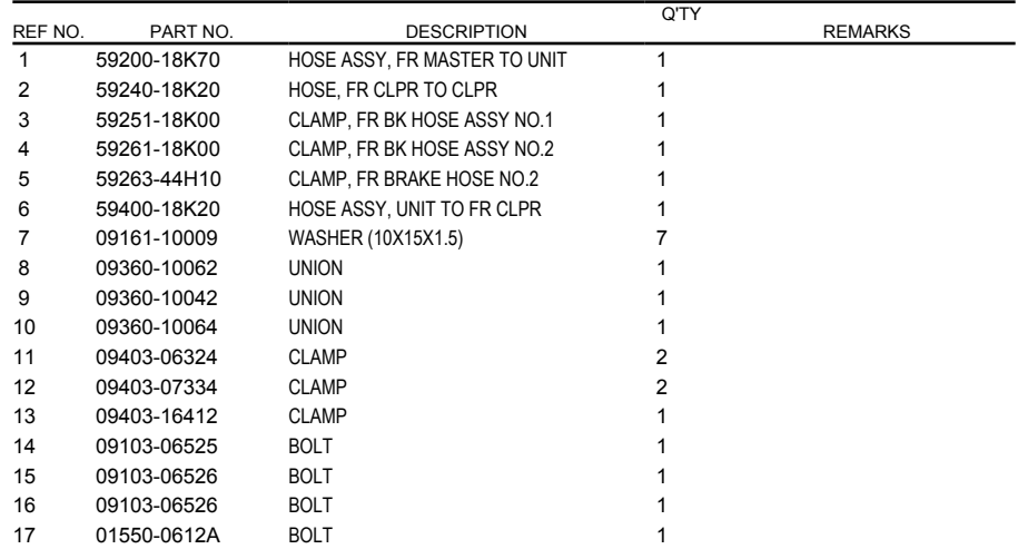
FIG.536H (2-G-7) FRONT BRAKE HOSE (SV650XAUL9 E19)
