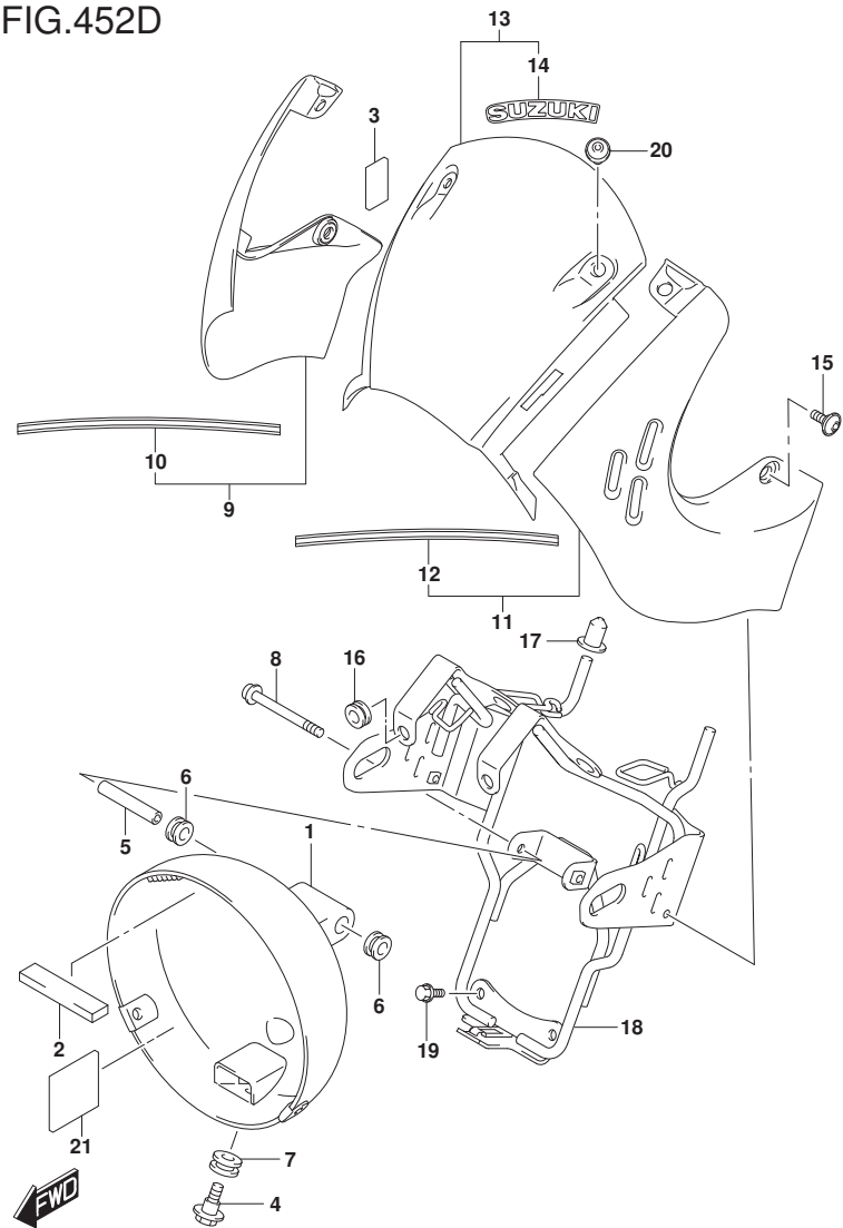
FIG.452D (2-B-4) HEADLAMP COVER (SV650XAL9 E19)
