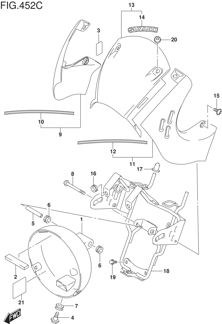
SV650AL9_E02_452C HEADLAMP COVER
