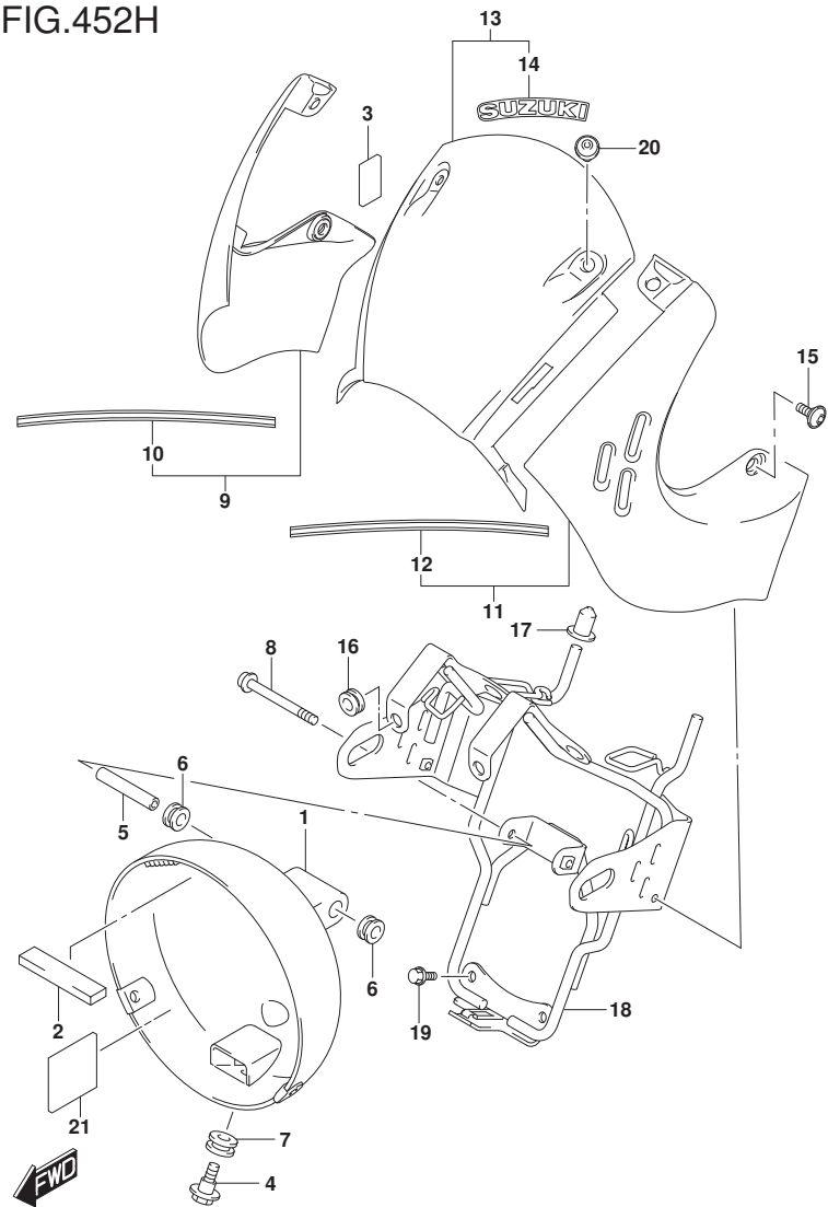
FIG.452H (2-B-8) HEADLAMP COVER (SV650XAL9 E19)
