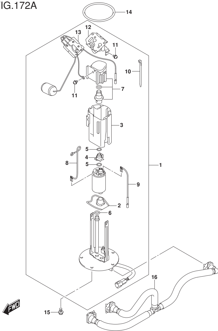
FIG.172A (1-C-3) FUEL PUMP
