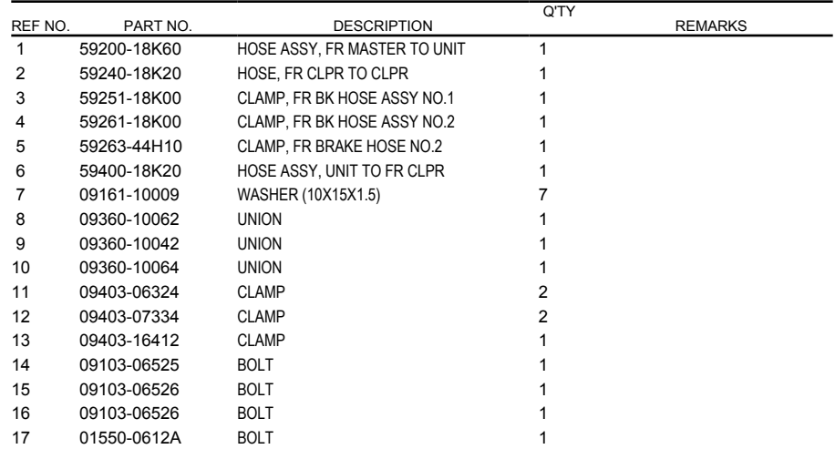
FIG.536A (2-F-14) FRONT BRAKE HOSE (SV650AL9 E02)
